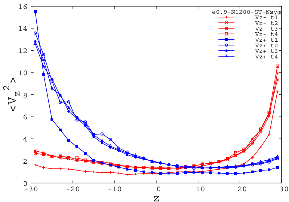
Figure 1.3 - 4: Simulations of granular gas is 3d rectangular cell
