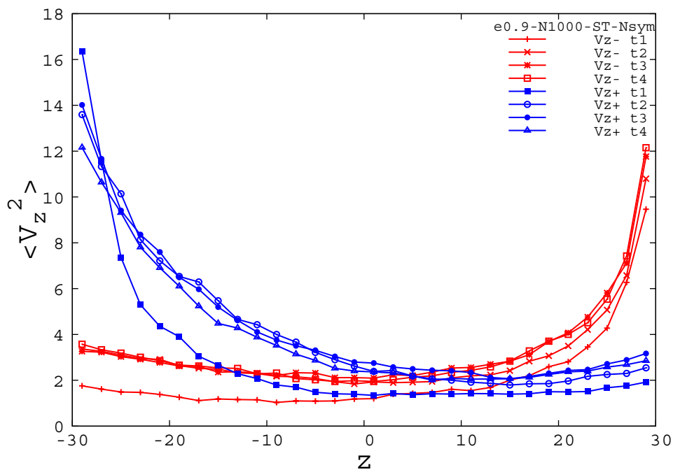
Figure 1.3 - 3: Simulations of granular gas is 3d rectangular cell
